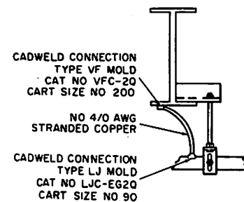
Figure 27. Recommended Typical Hanger Installation
