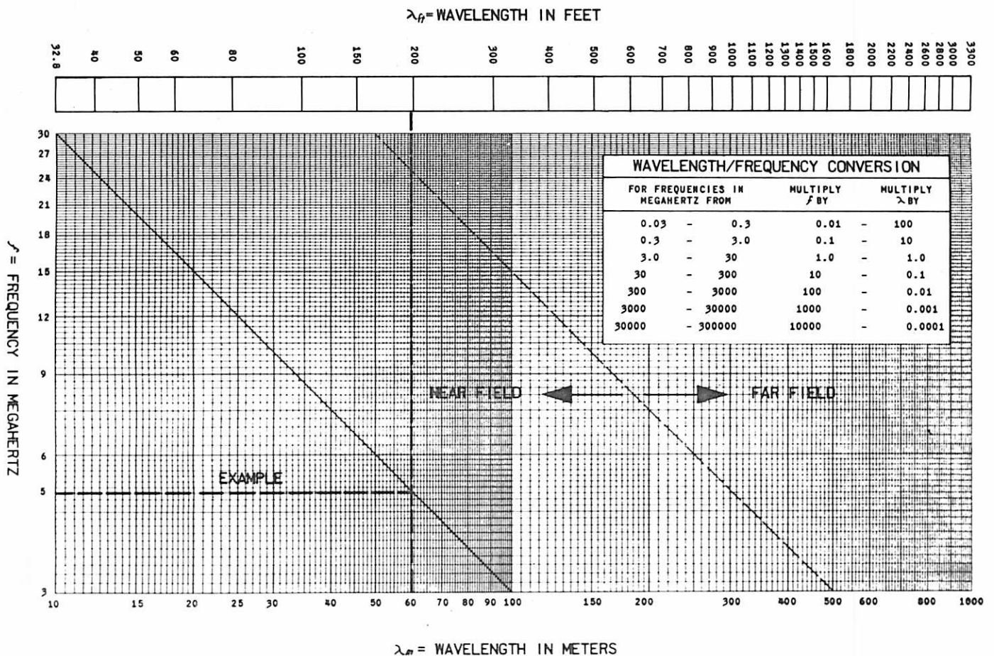
Figure 2. Wavelength/ Frequency Conversion
