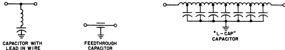
Figure 12. Electrical Circuit Equivalents for Capacitor Suppression Devices
