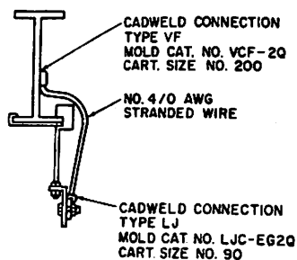
Figure 26. Recommended Beam Support for Ground Bus
