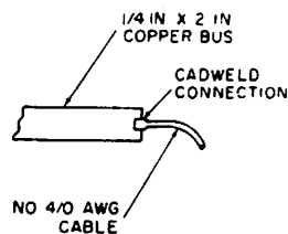
Figure 30. Preferred Connection of Bus Bar to the End of a Bus Bar
