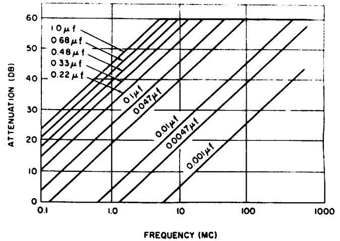
Figure 18. Insertion Loss Curves of a Feedthrough Capacitor
