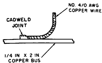
Figure 28. Recommended Terminal Connection
