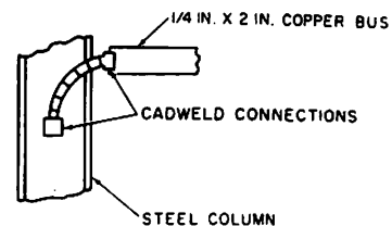
Figure 29. Preferred Column Connection
