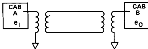
Figure 8. A Balanced Line for Reducing Susceptibility to Interference
