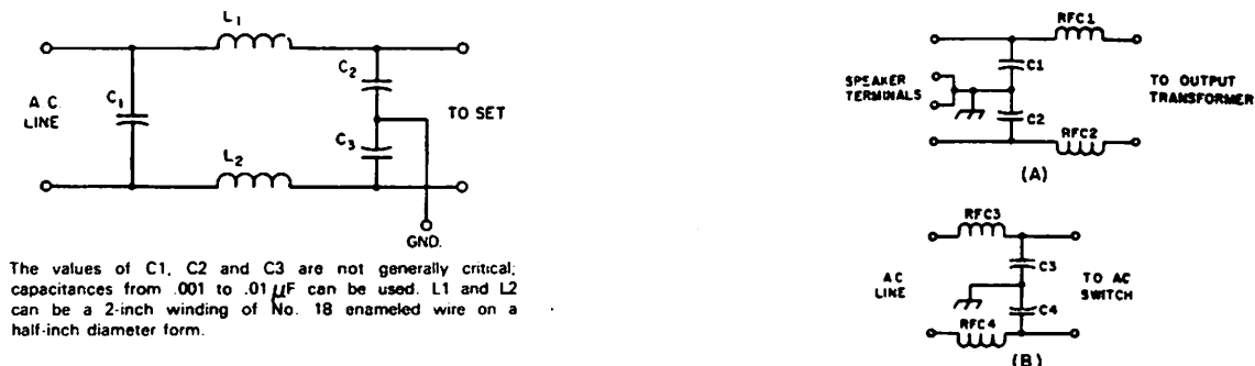
Figure 20. "Brute-force" ac Line Filter
