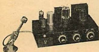
SIGNET 10 ASSEMBLY
