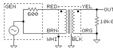
TEST CIRCUIT 3
