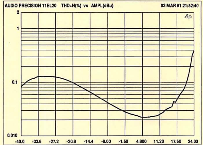
RE-11-ELCF 20Hz DISTORTION
