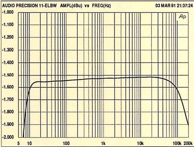
RE-11-ELCF MAGNITUDE RESPONSE
