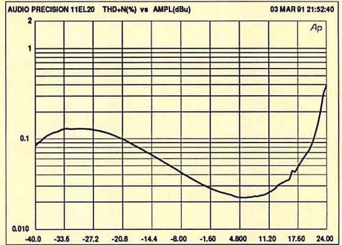
RE-123-ELCF 20Hz DISTORTION
