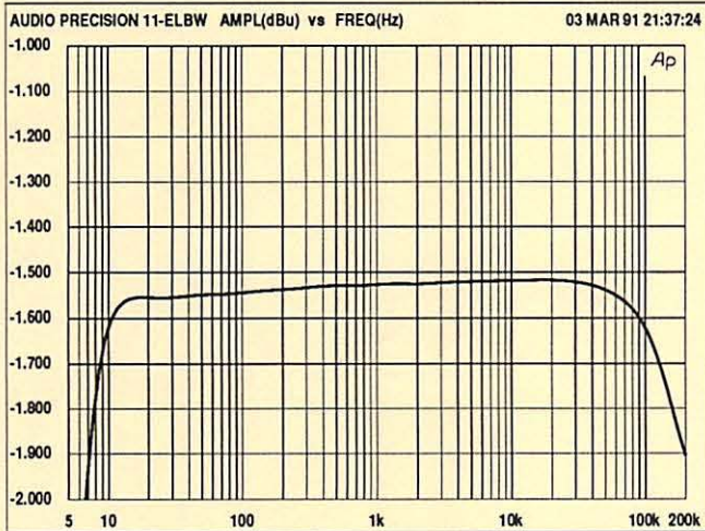
RE-123-ELCF MAGNITUDE RESPONSE
