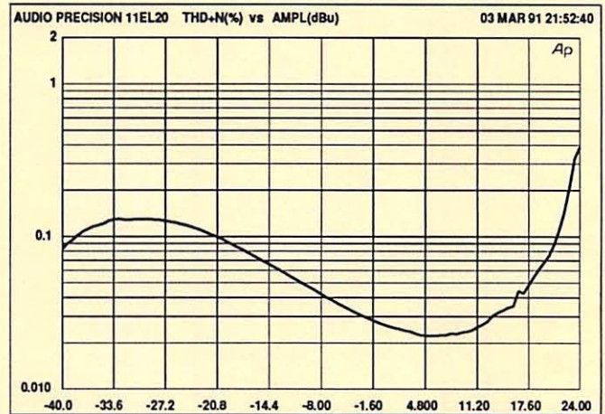
RE-123-ELPC 20Hz DISTORTION
