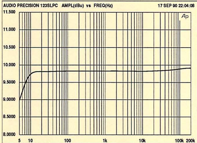
RE-123-ELPC MAGNITUDE RESPONSE
