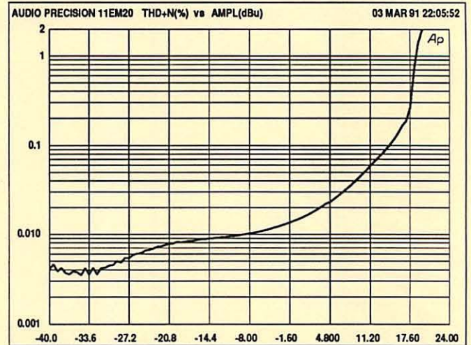
RE-123-EMCF 20Hz DISTORTION
