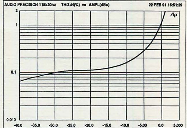
RE-115K-E 20Hz DISTORTION
