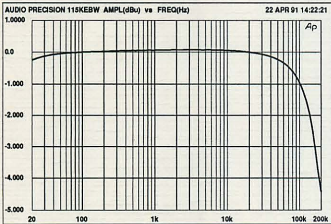
RE-115K-E MAGNITUDE RESPONSE
